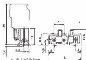
2-24通道弯型焊针插座(防错) KF475-R/KF478-R
