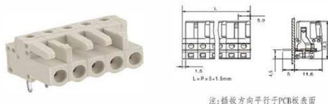
2-24通道孔型插头带弯型焊针 (防错)
