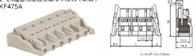
2-24通道孔型连接器带卡接钩 (防错) KF475A
